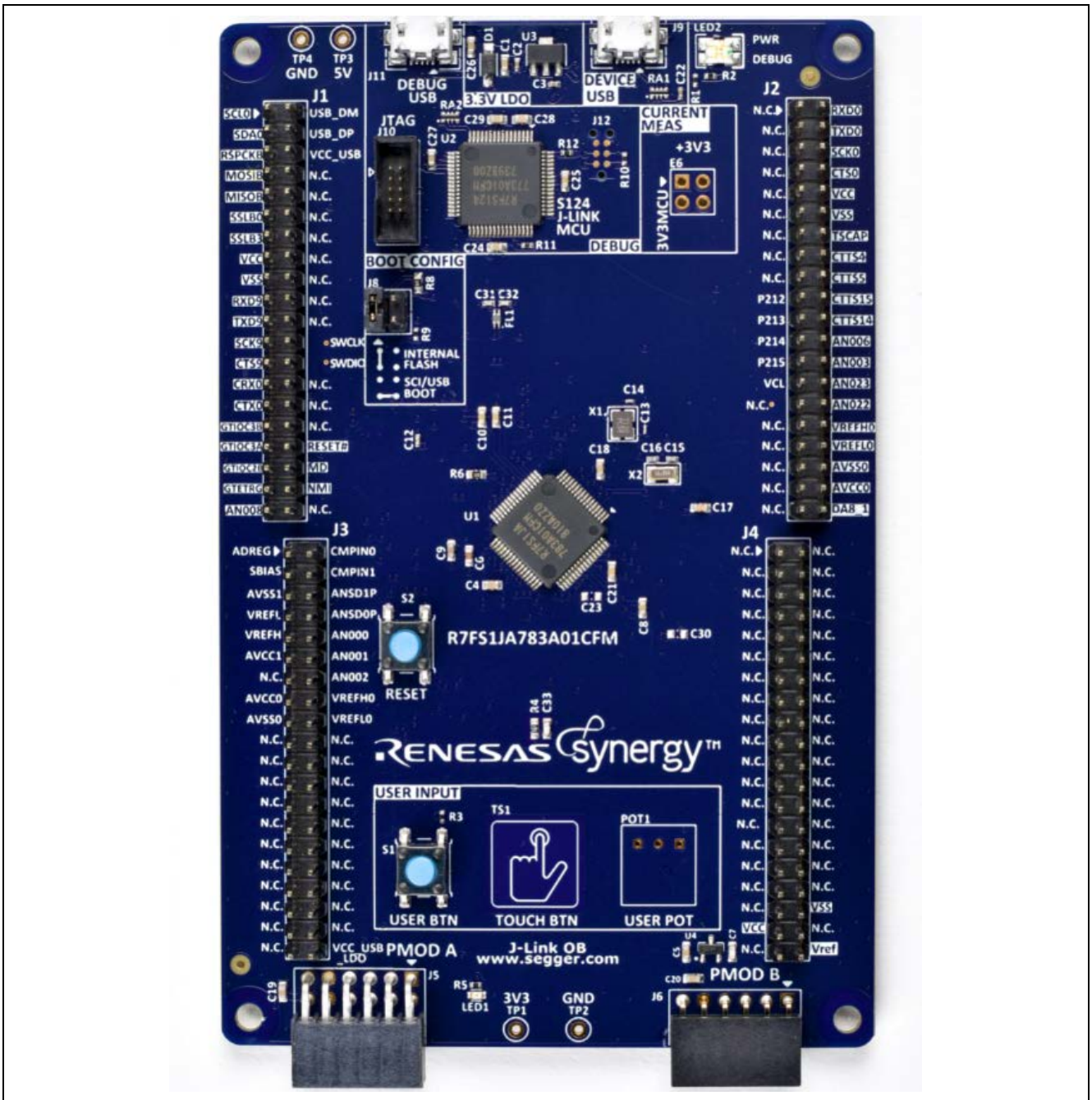
Figure 1 TB-S1JA Board
